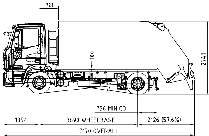
URBIN 11m WITH UNDERBODY LIFTER
