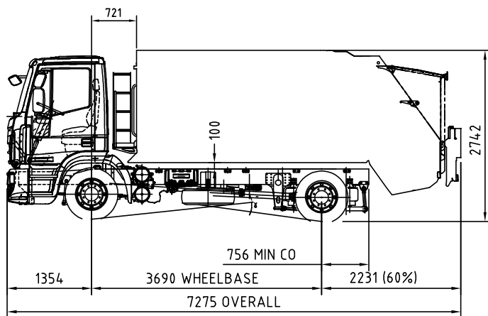
URBIN 11m WITH UCBL LIFTER
